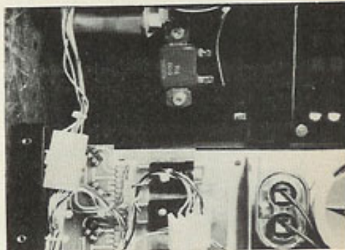
Fig. 9—Tape control pushbuttons are attached to the rear of a printed circuit card (bottom-left). Take-up reel motor is at top, with ballast resistor and capacitor on swing-away panel at left.
