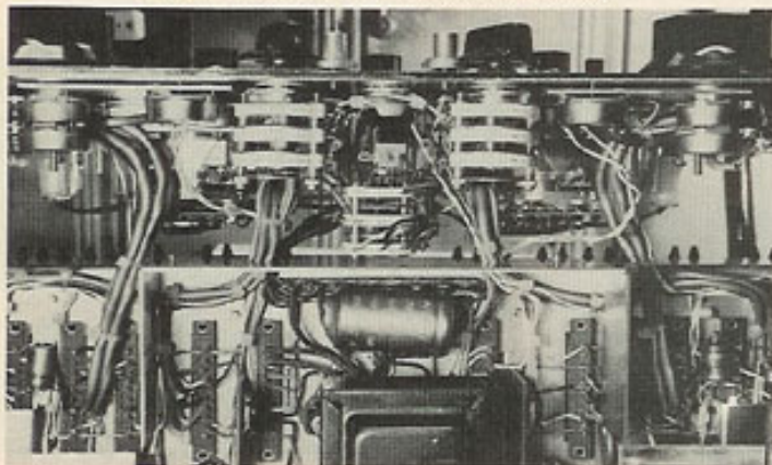
Fig. 11—Underside of electronics chassis.
