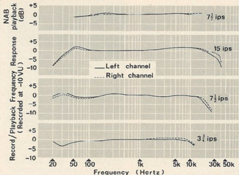
Fig. 10—Record/playback response of Crown CX822 stereo tape recorder.
